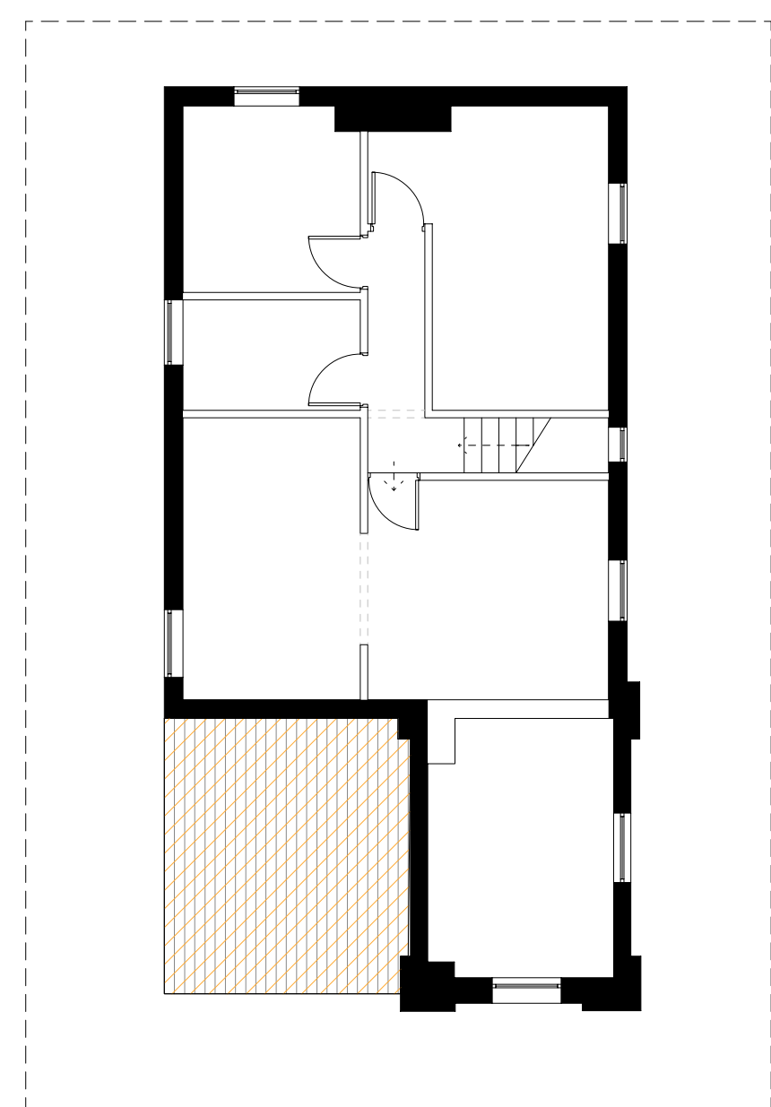
COTTAGE AND TOWER - FIRST FLOOR
