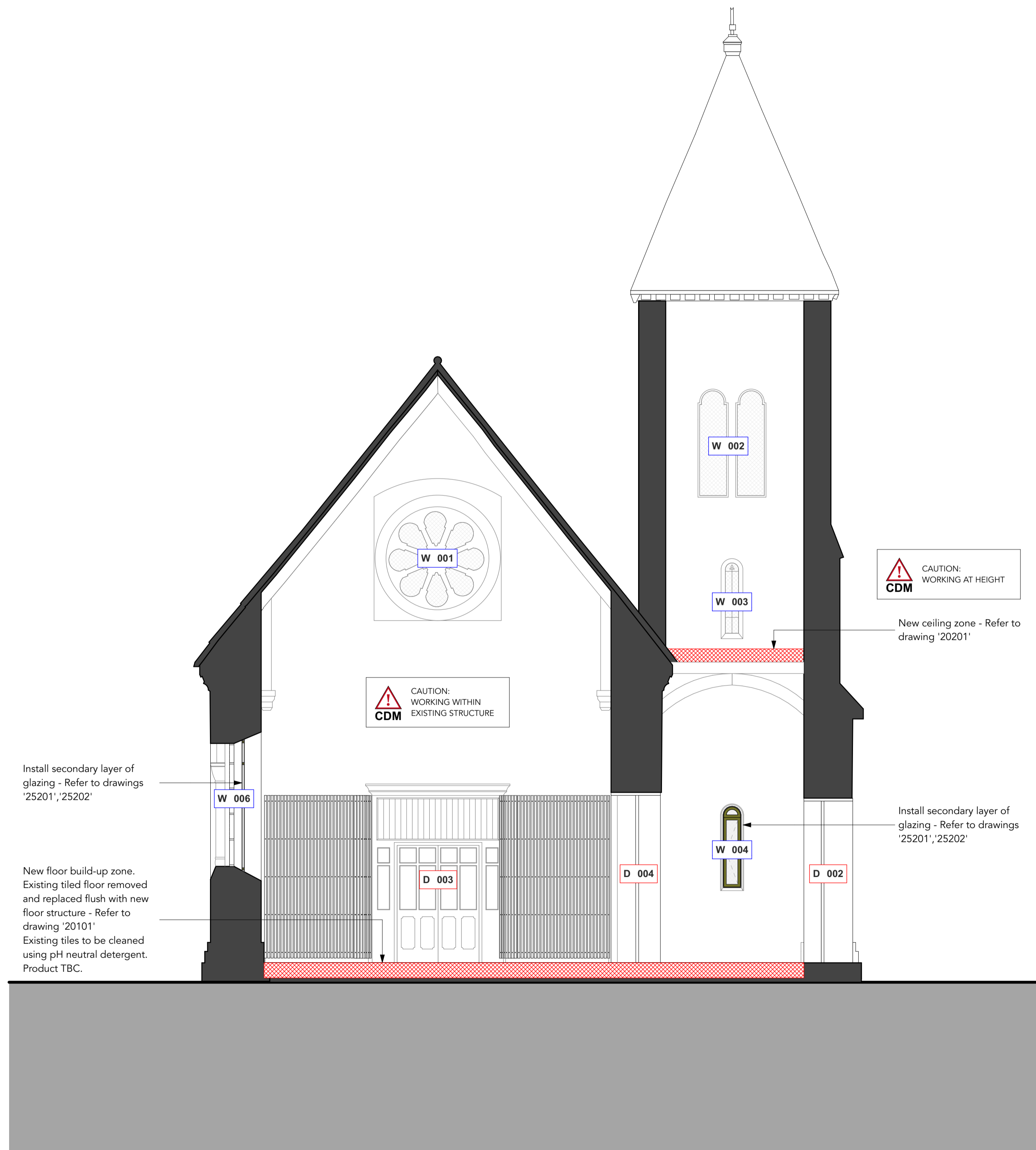
Anglican Chapel Section AA Proposed
