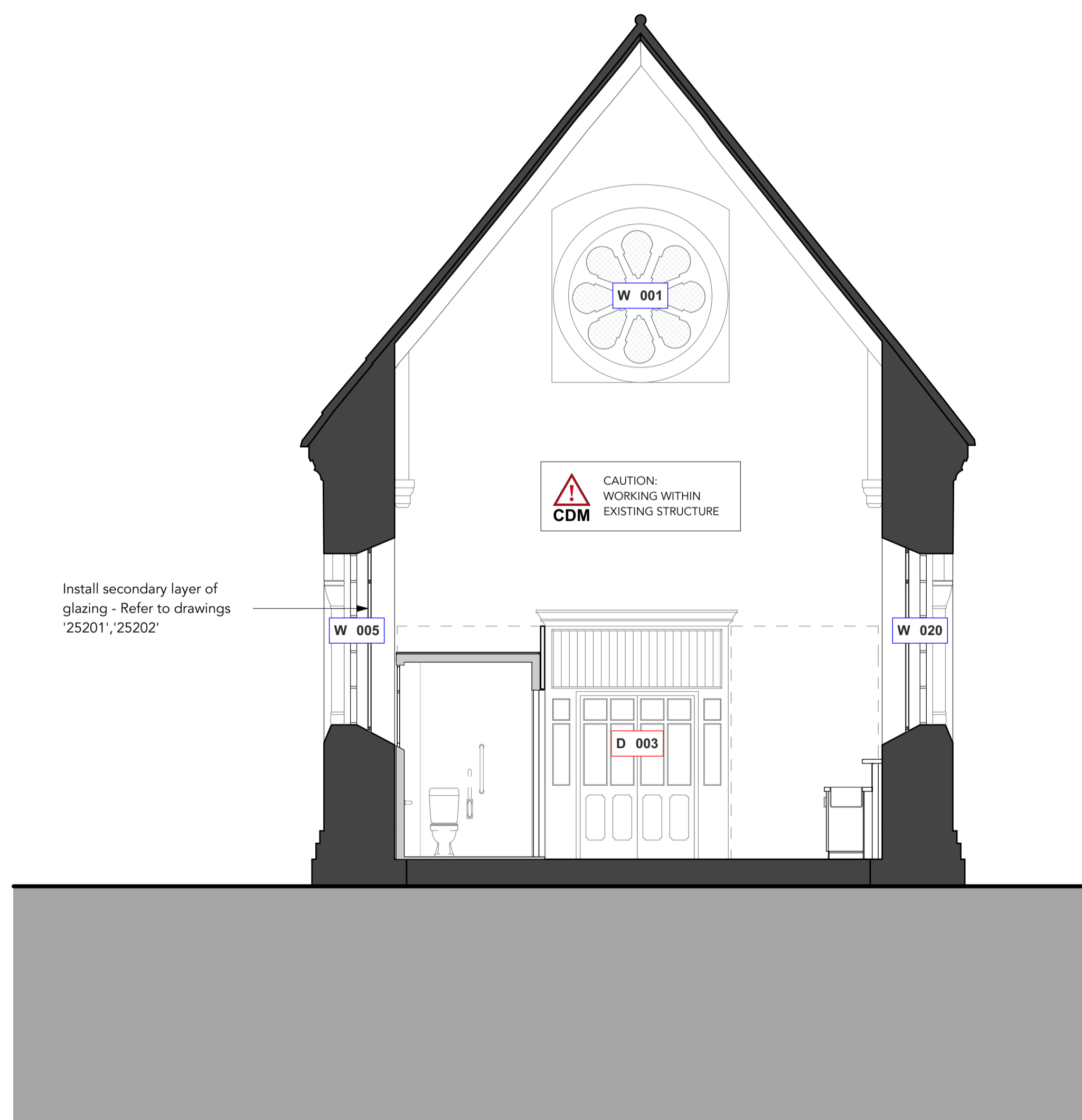
Anglican Chapel Section BB
