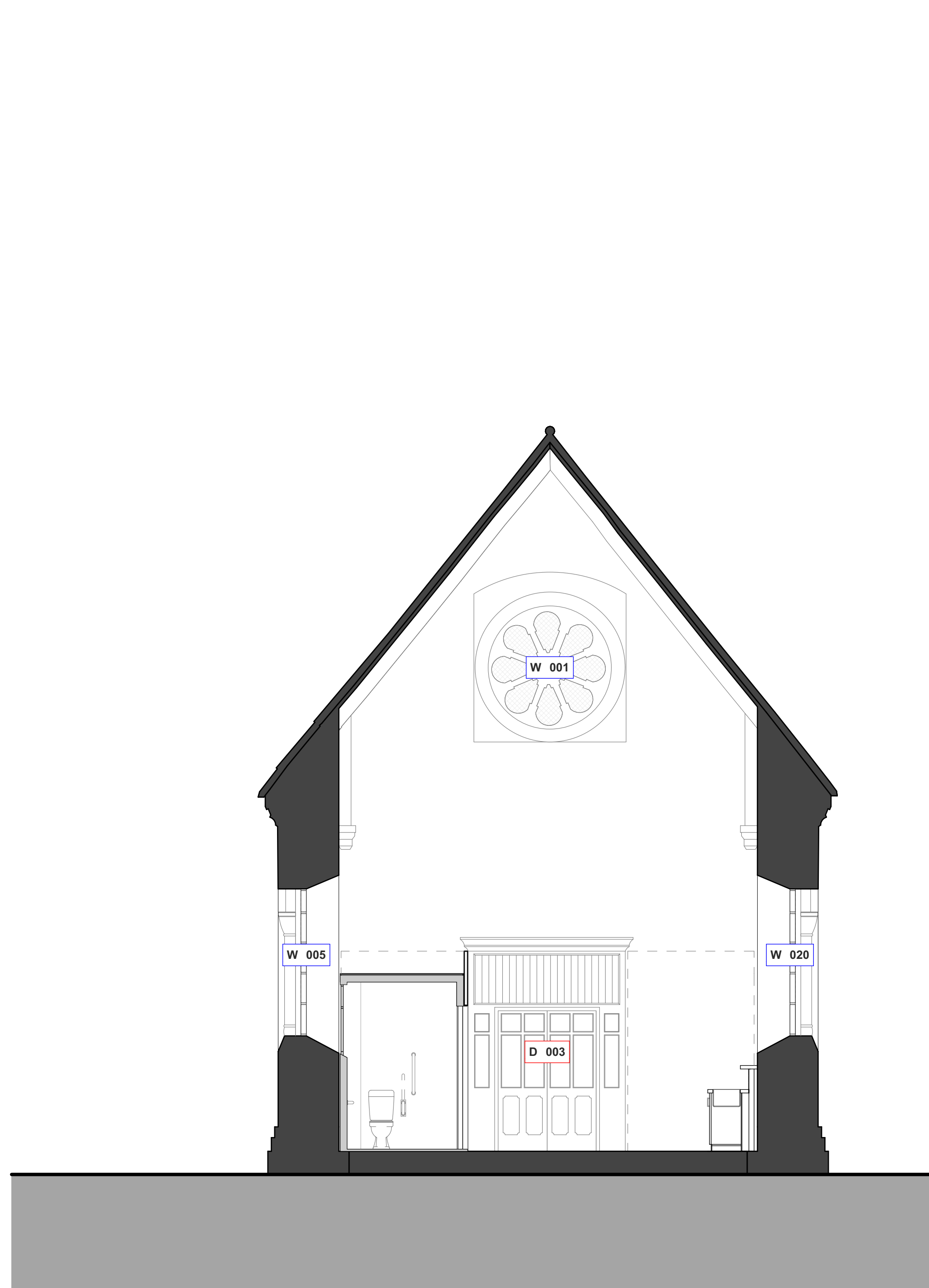
Anglican Chapel Section BB
