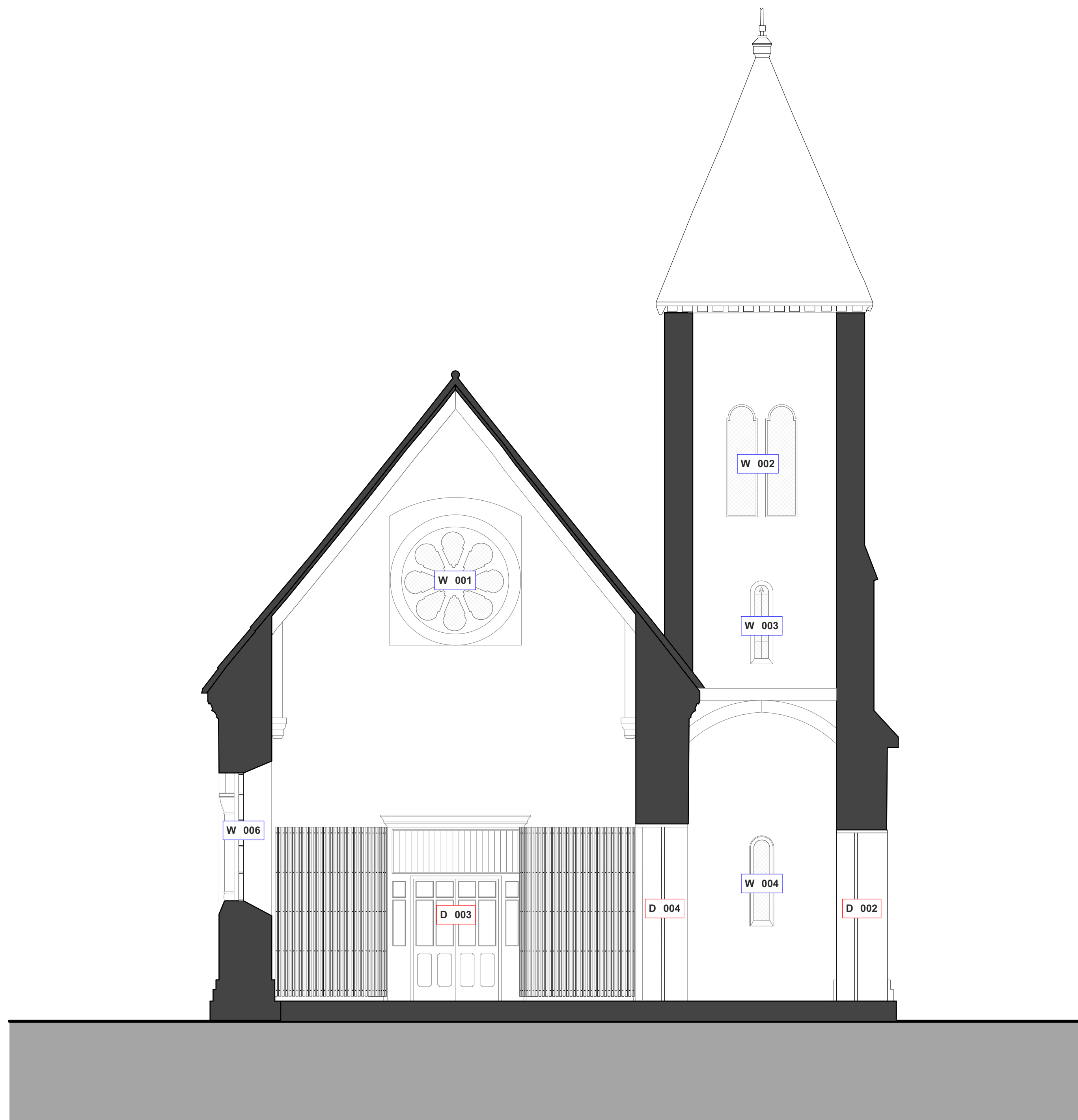
Anglican Chapel Section AA Existing
