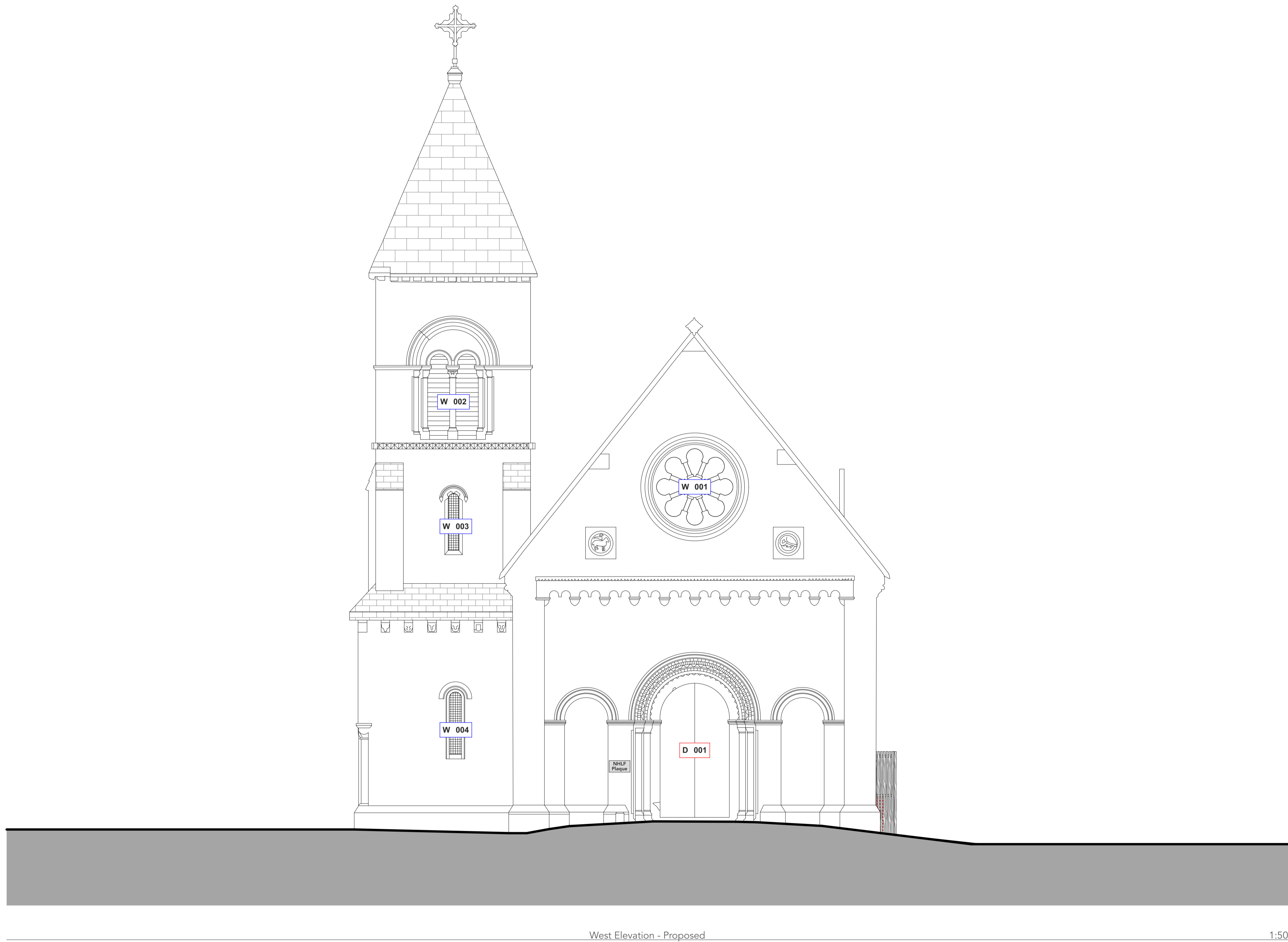
West Elevation - Proposed
