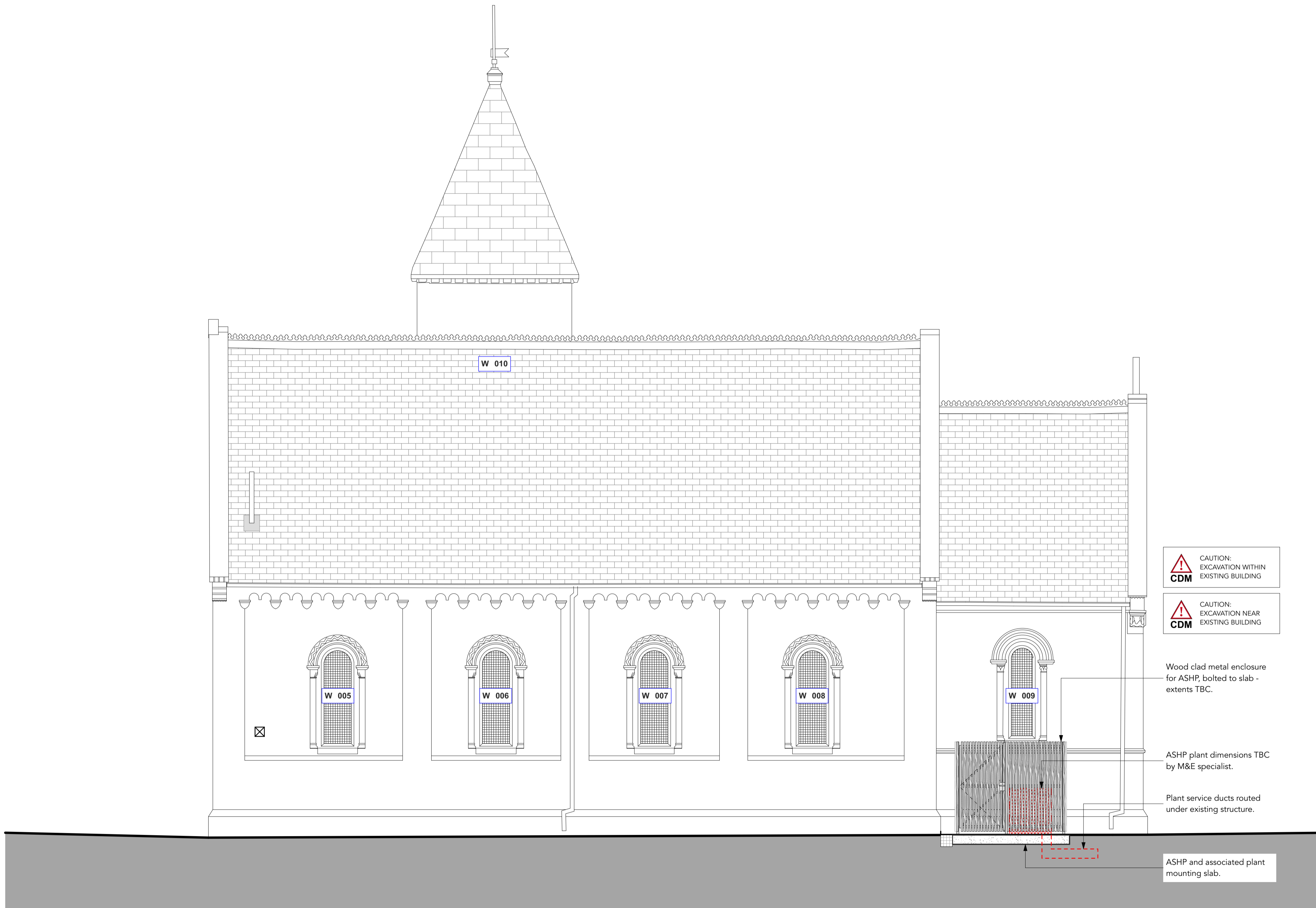
South Elevation - Proposed
