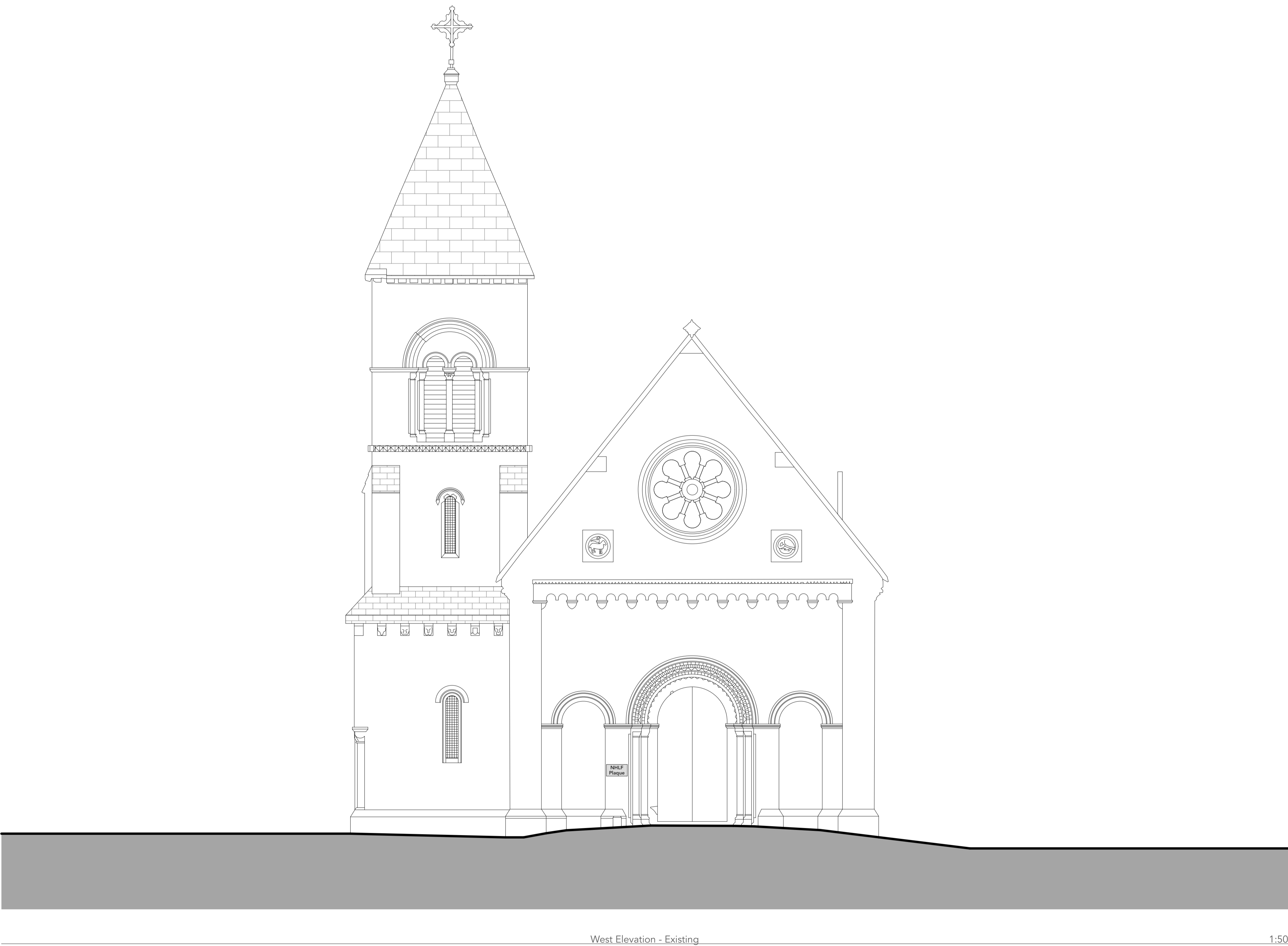
West Elevation - Existing
