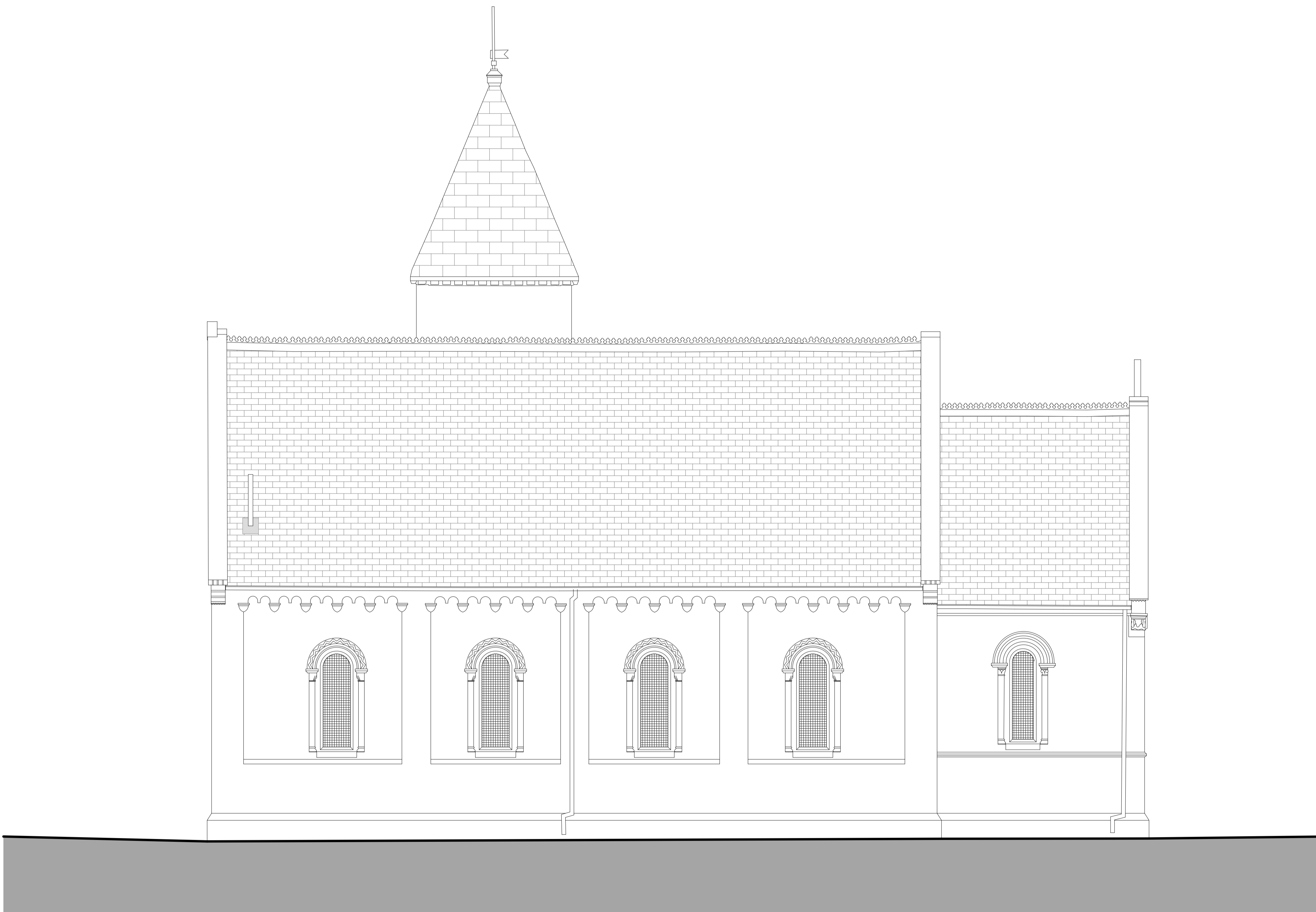
South Elevation - Existing
