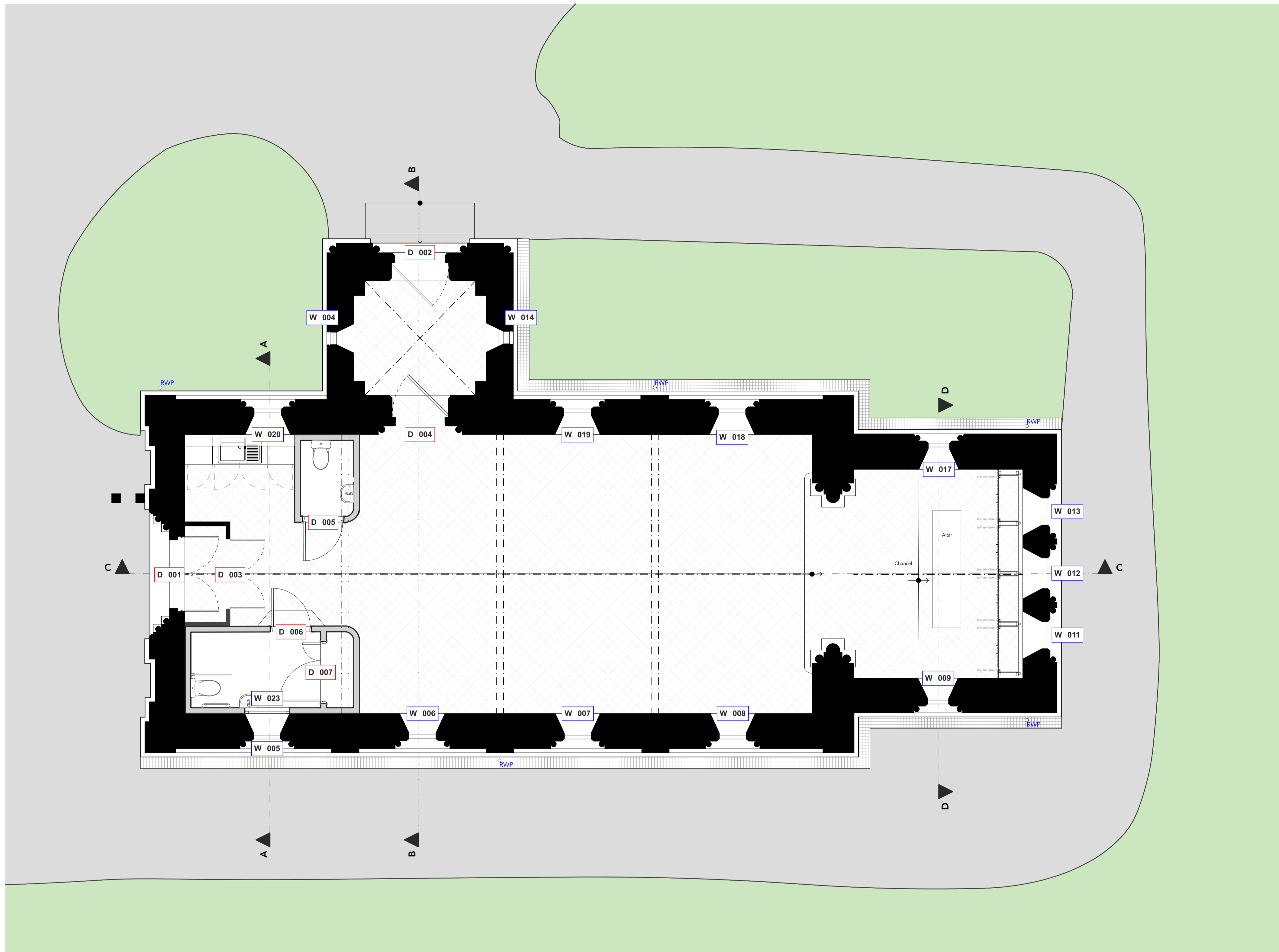
Anglican Chapel Ground Floor Existing
