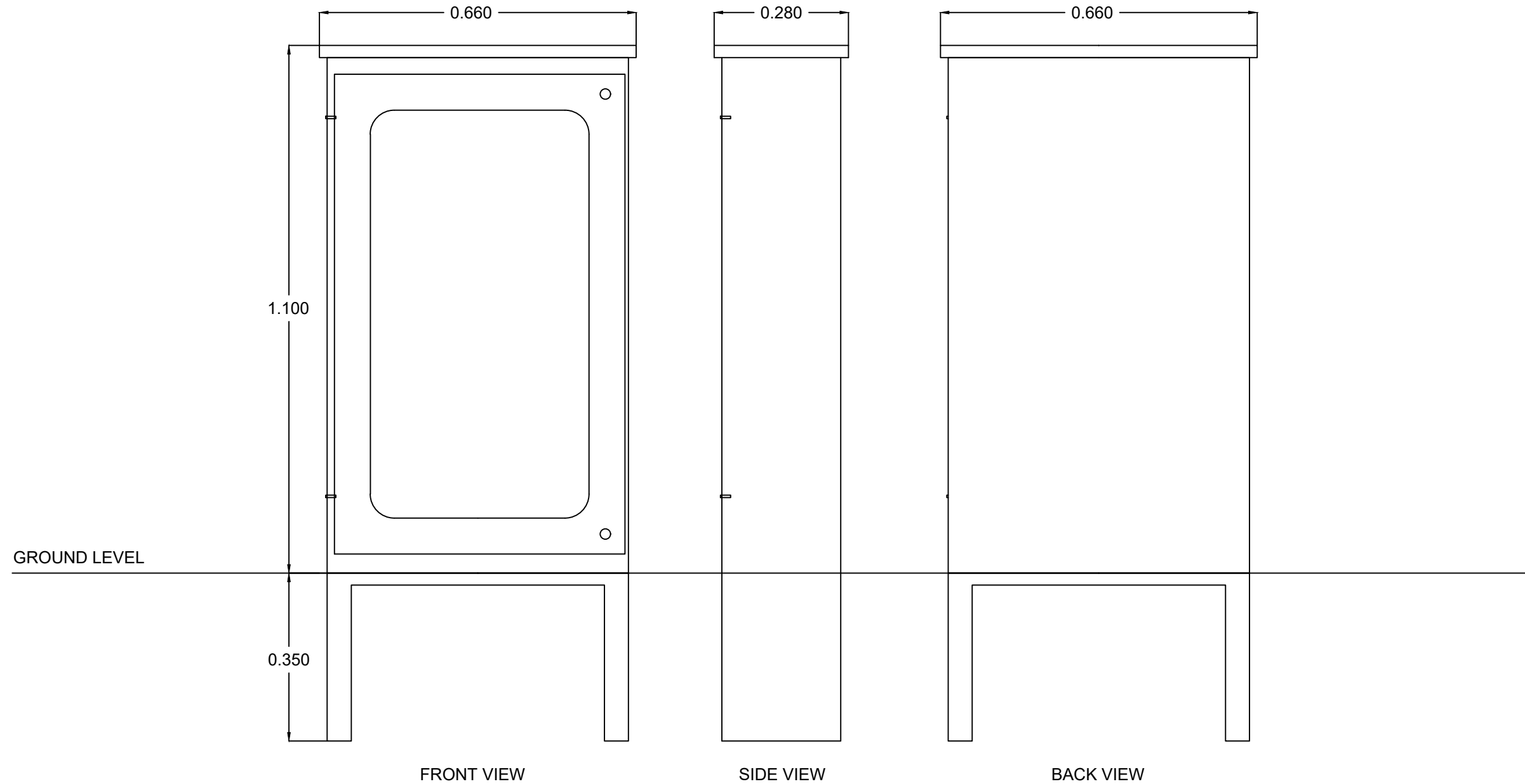
ELEVATION PLAN CABINET SCALE 1:10
