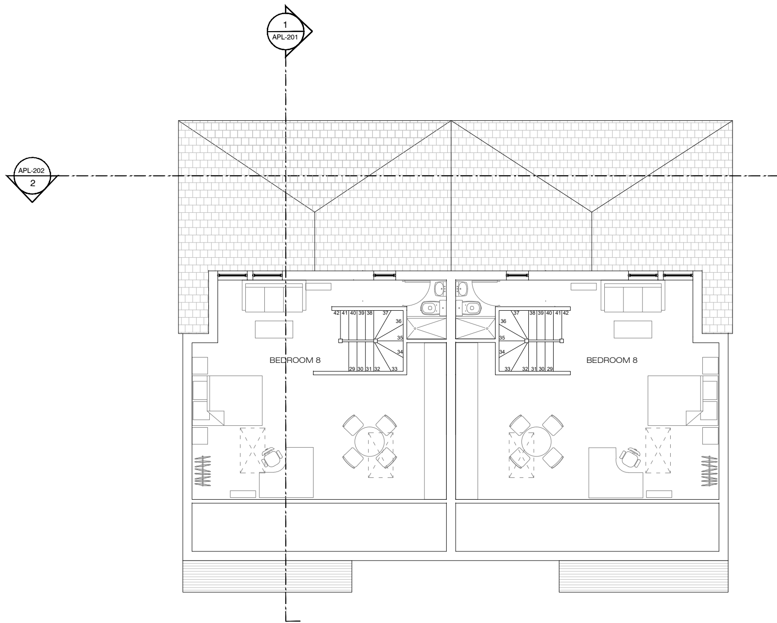
01 Second Floor scale: 1:50
