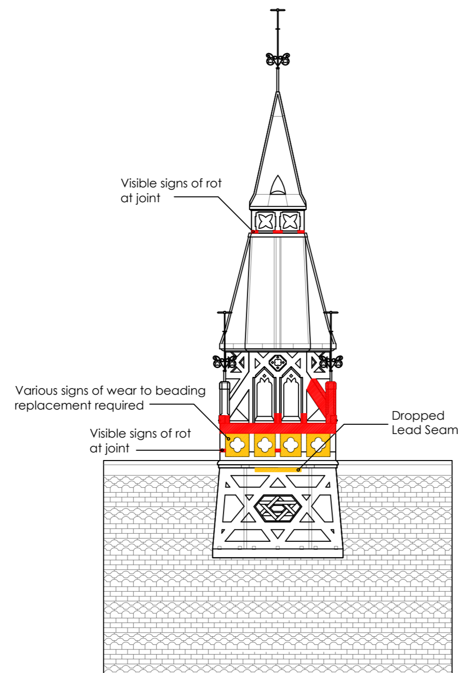
East Elevation
