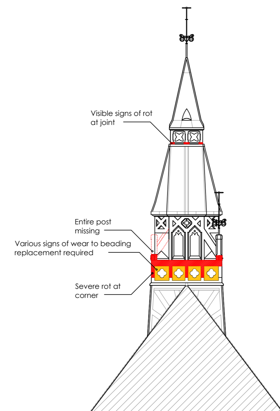
South Elevation
