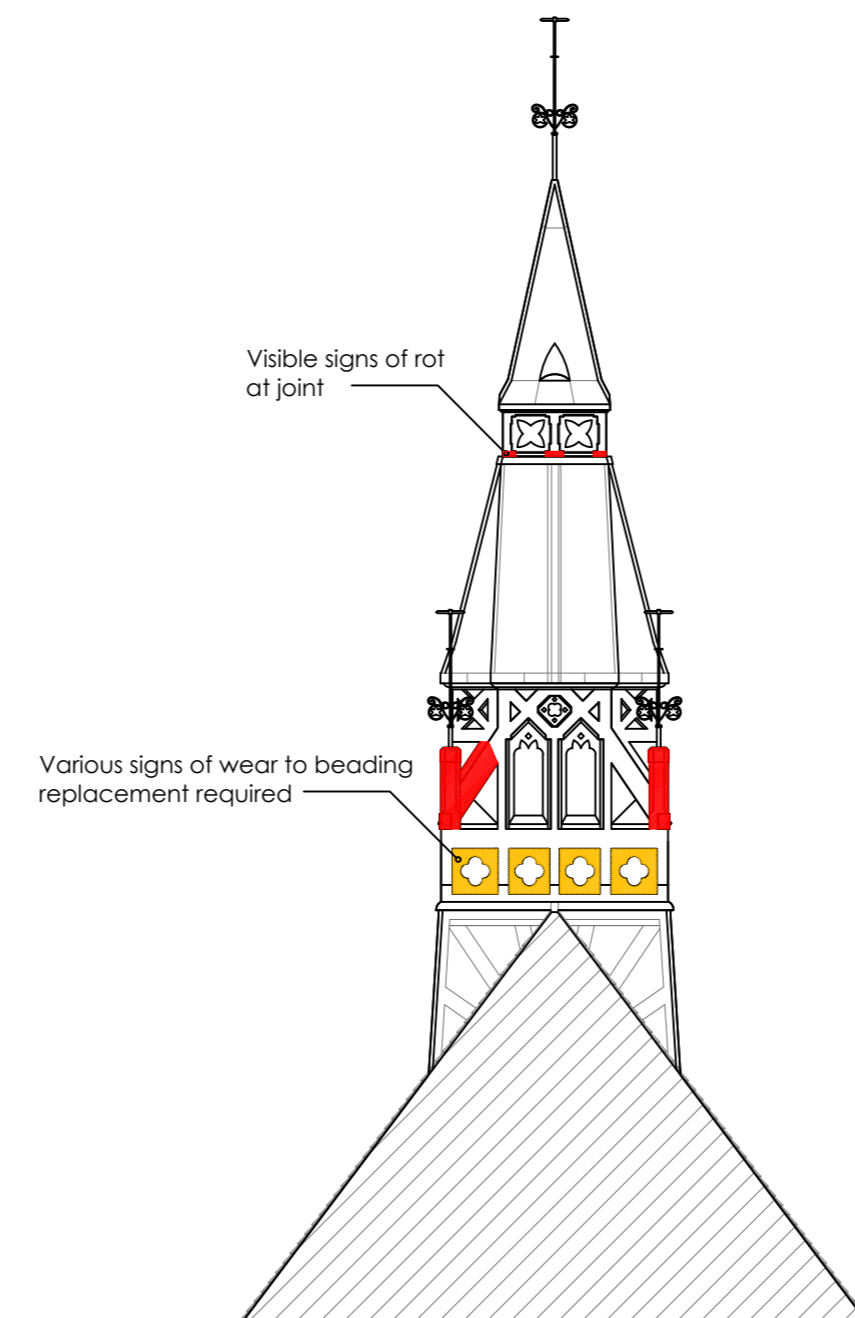
North Elevation
