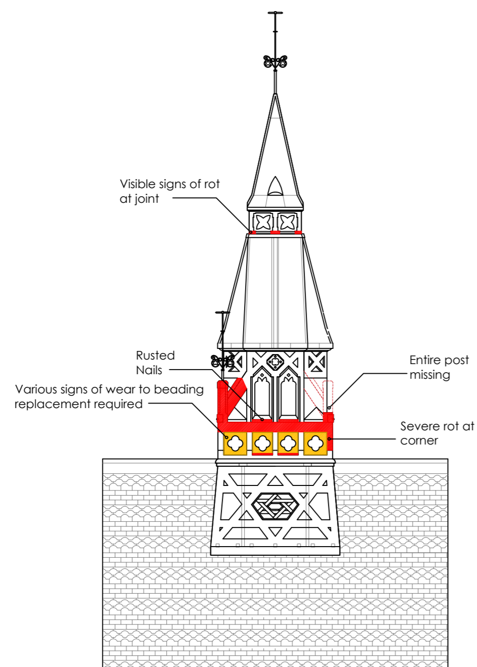
West Elevation
