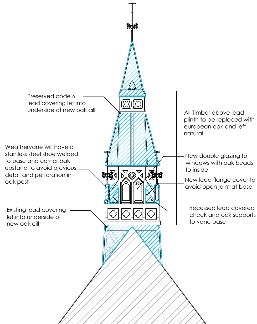
North & South Elevation
