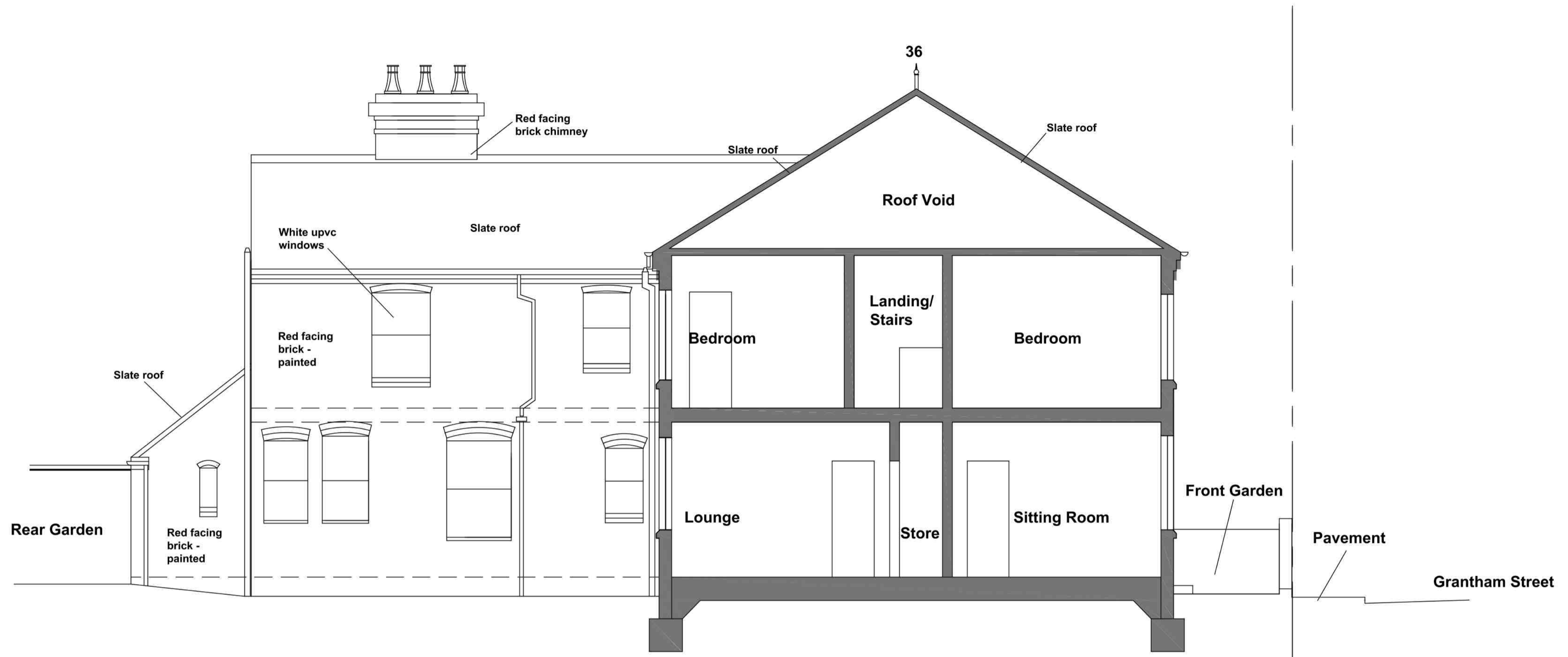
Existing Section AA Scale 1:50 @ A1
