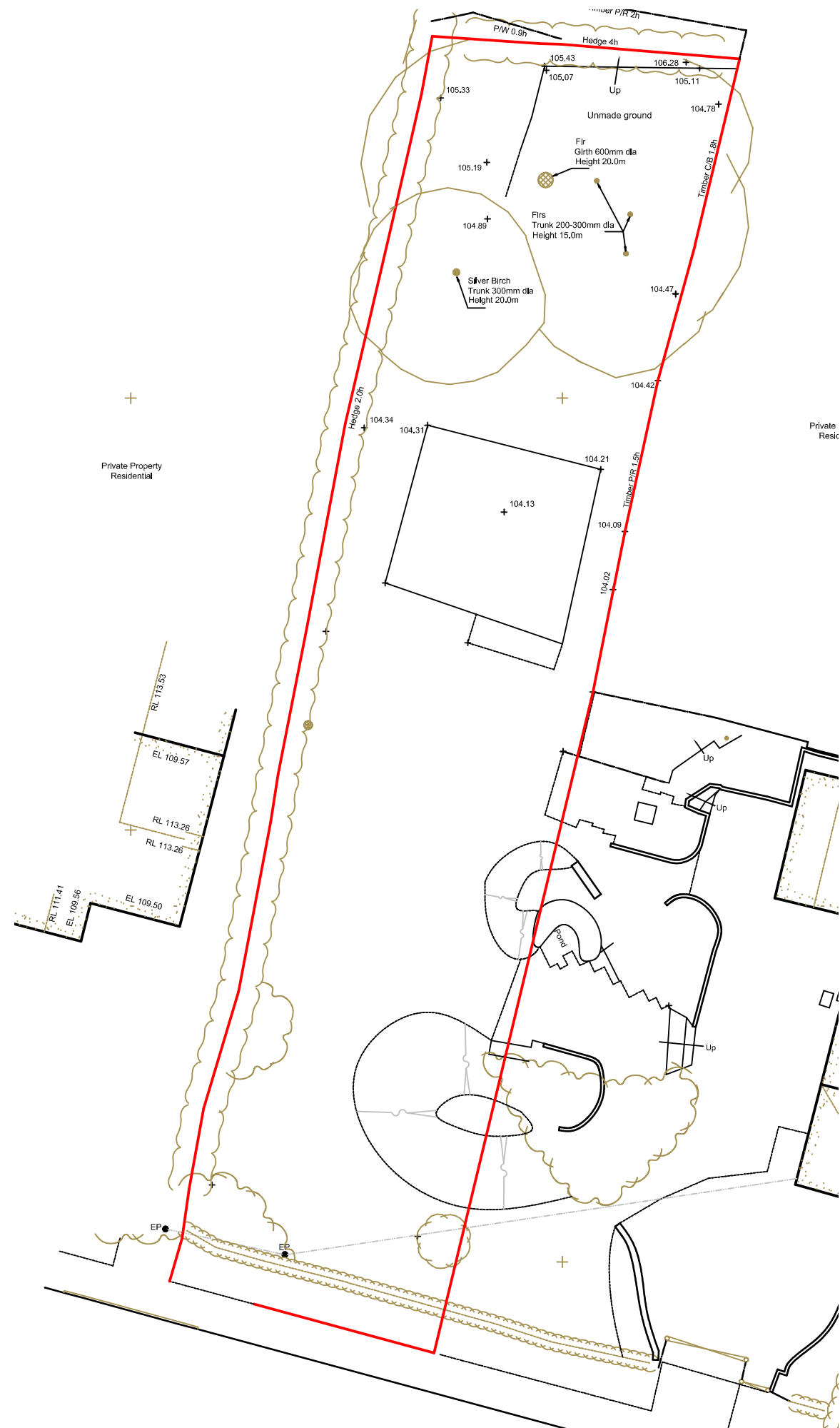
TREE SURVEY PLAN 1:250 @ A3
