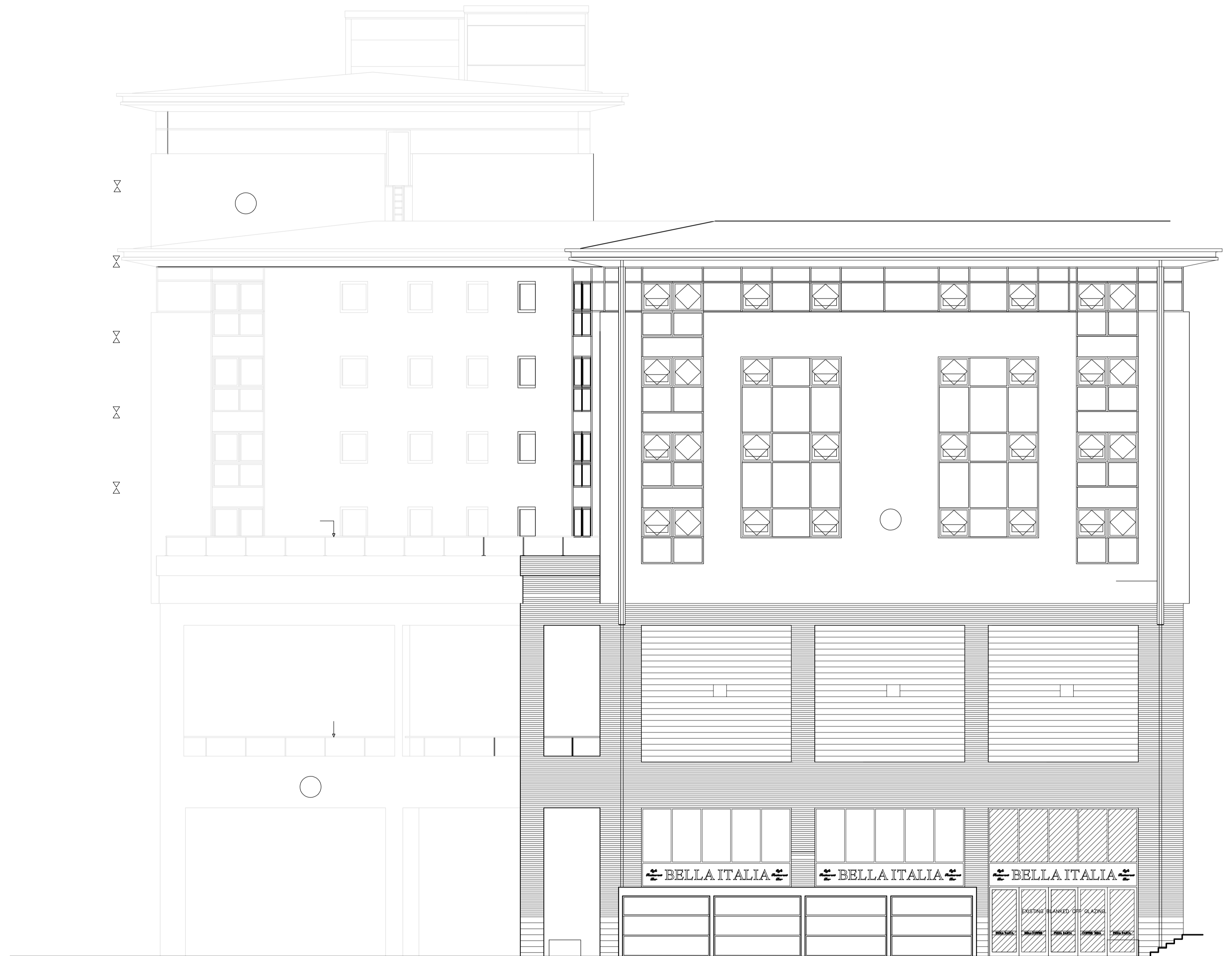
SOUTH EAST (FRONT) ELEVATION
