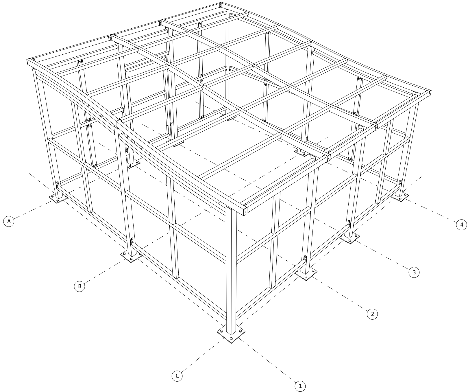
3-D VIEW
