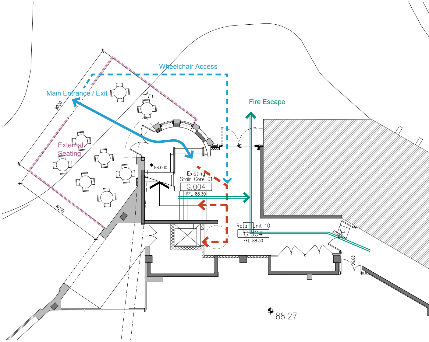
Lower Ground Floor - As Proposed
