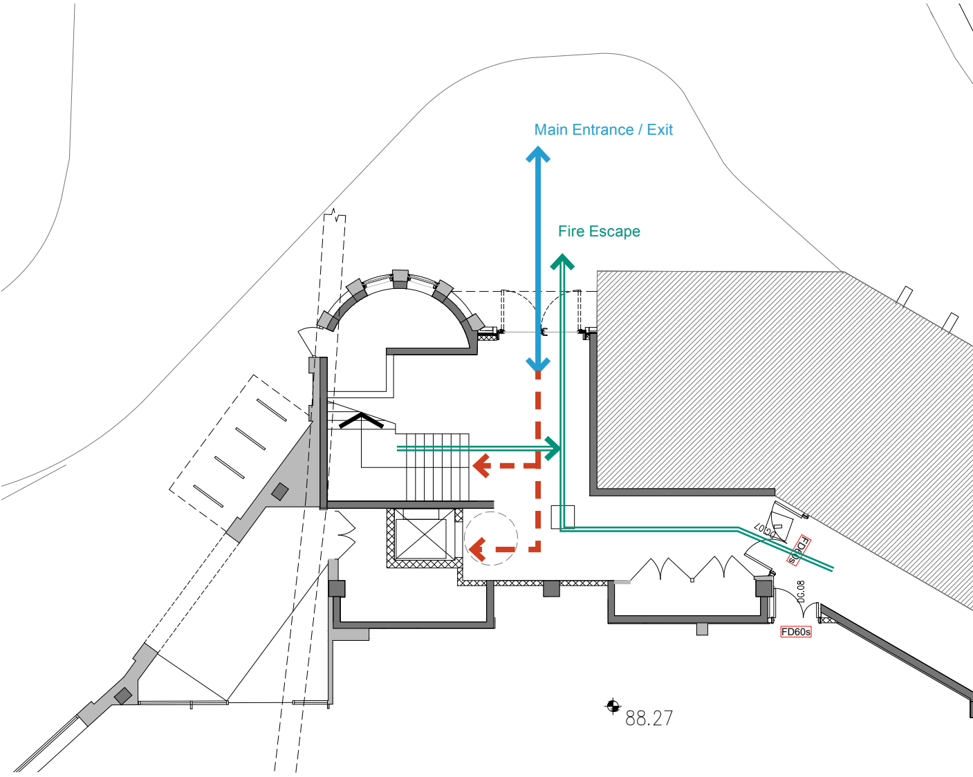
Lower Ground Floor - As Approved
