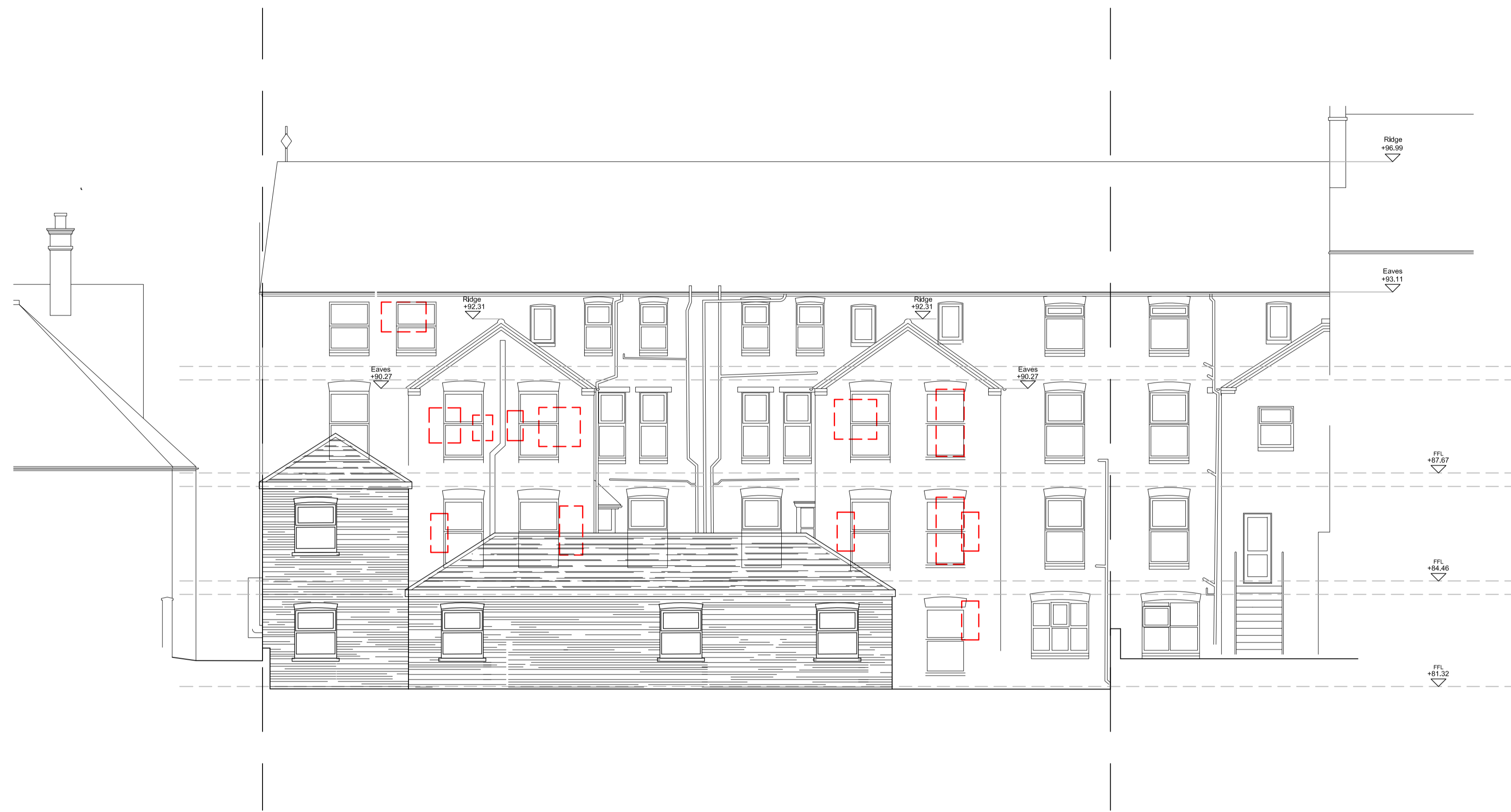
REAR ELEVATION
