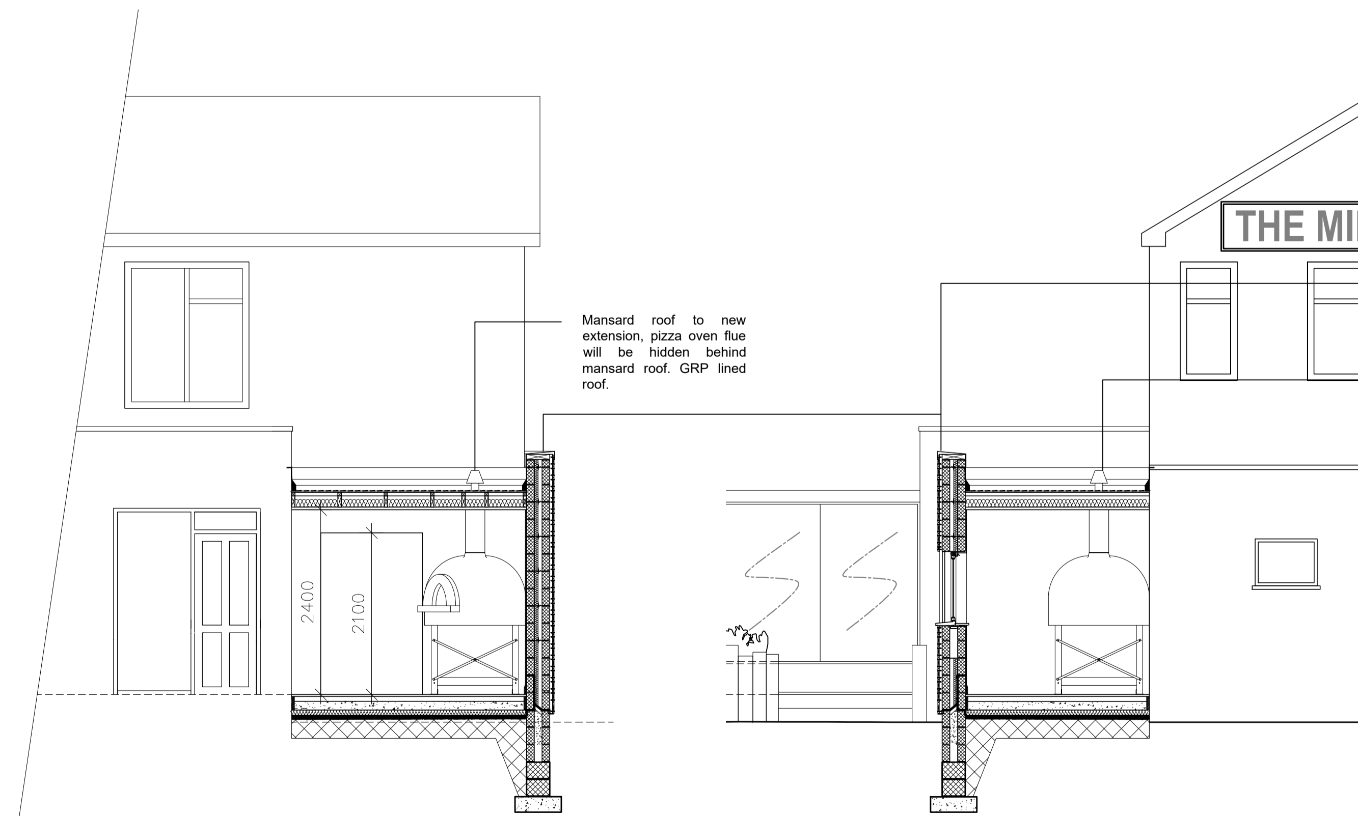
PROPOSED SECTION: A 1:50@A1
