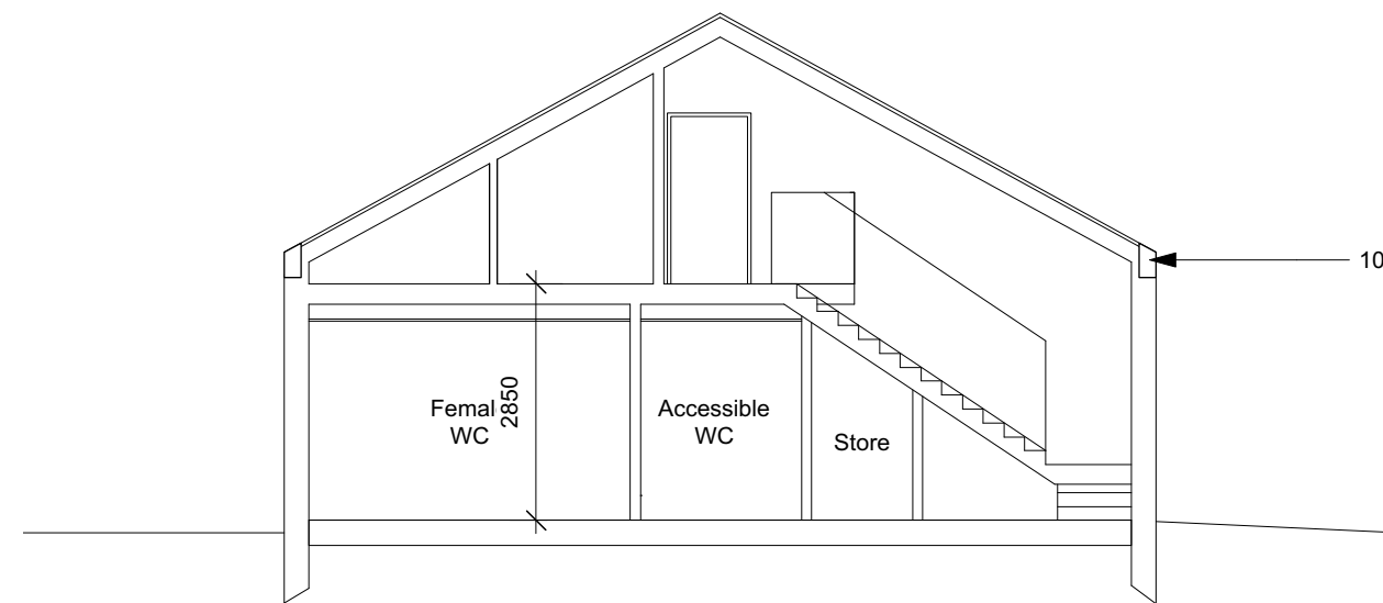
02 PROPOSED SECTION B 1:100
